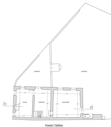
PIANO TERRA
